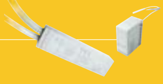
Tag system Concealed and feedthrough installing radio control systems made up of a TTX4 transmitter and TT1 and TT2 control units. Ideal to manage any home automation, lighting point and load up to 500 W
